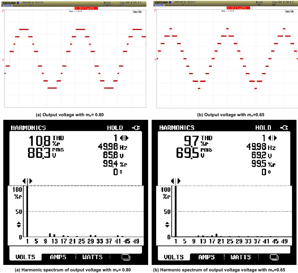
FIGURE 8. Output voltage waveform and their respective harmonic spectrums for 9 levels in symmetrical configuration.
