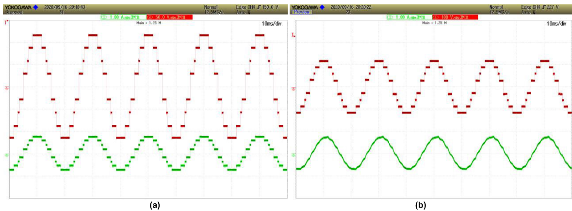
FIGURE 9. Output voltage and current with symmetrical configuration (a) R load and (b) RL load, and with asymmetrical configuration.
