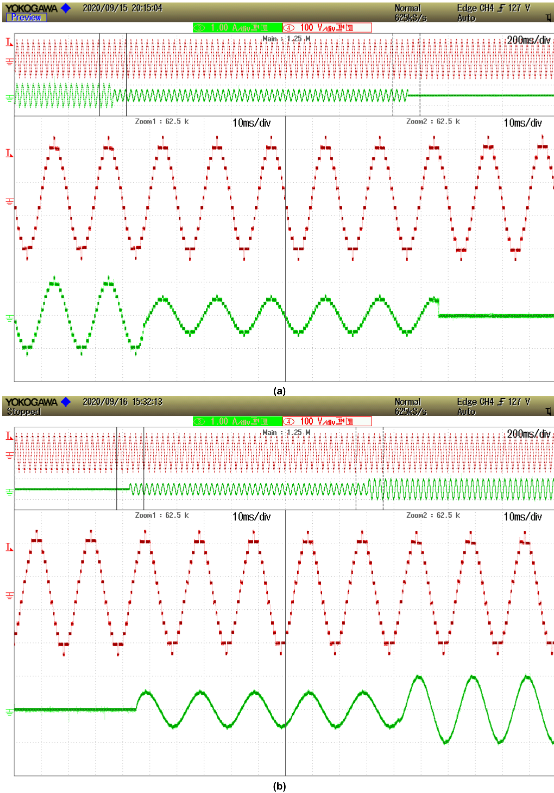
FIGURE 13. Output voltage and current waveform with change in (a) R load and (b) RL load with asymmetrical configuration.
