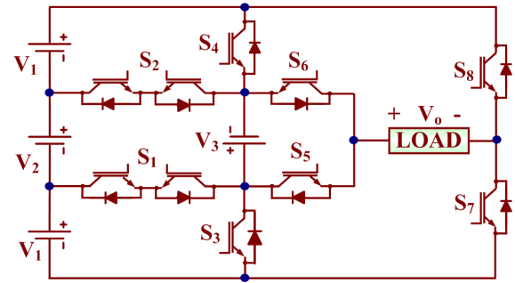
FIGURE 1. Power Circuitry of the Basic unit of proposed topology.
