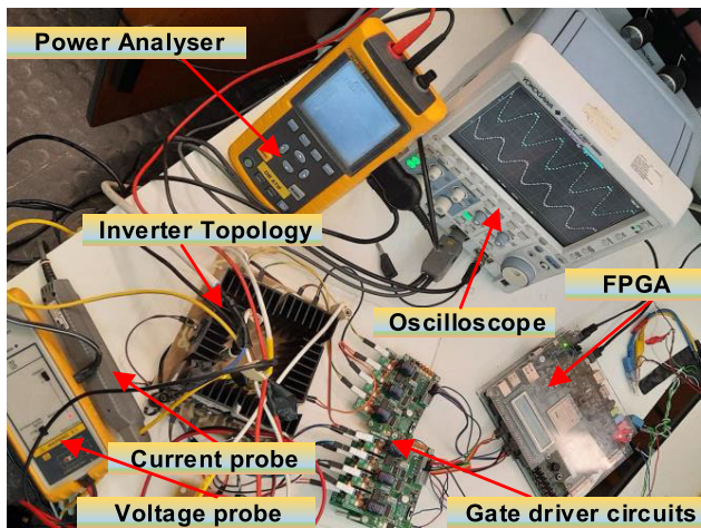
FIGURE 7. Hardware setup of the proposed MLI.
