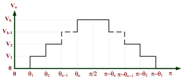
FIGURE 3. Staircase output voltage.
