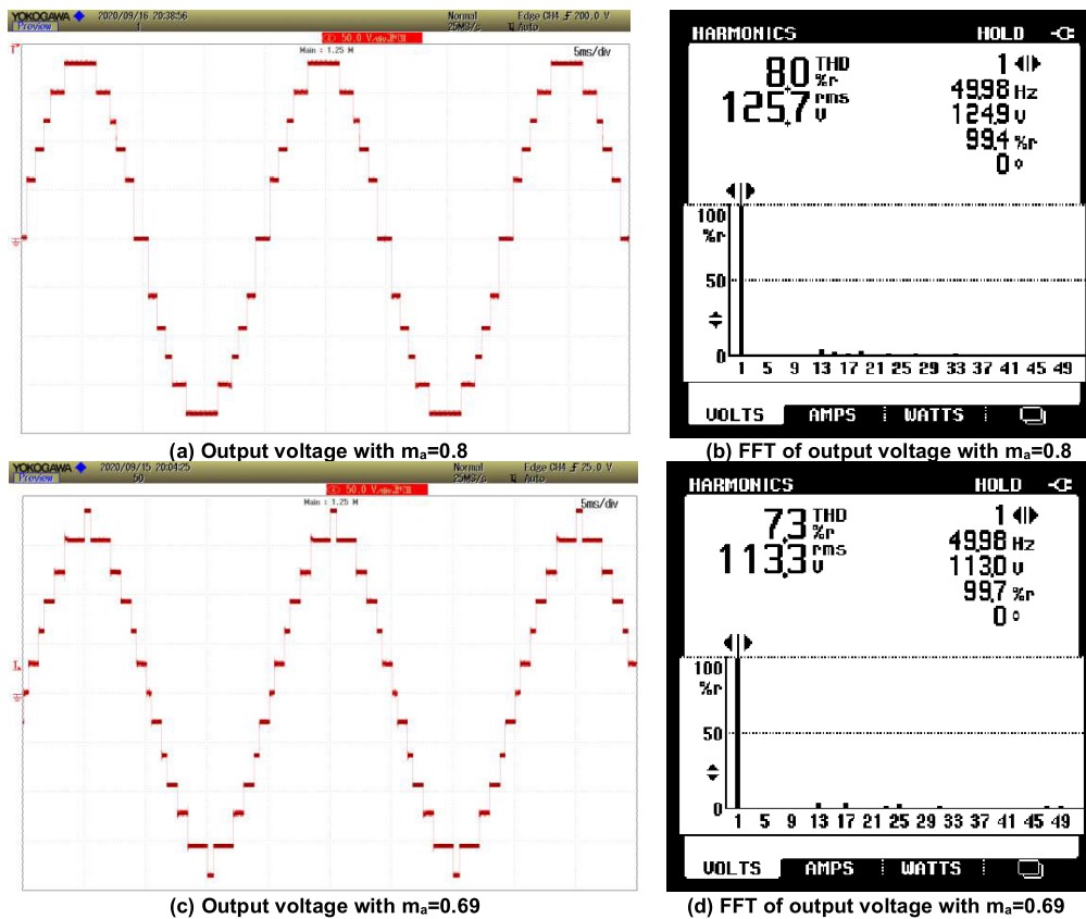
FIGURE 12. Output voltage and FFT of output voltage for asymmetrical configuration.
