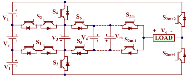
FIGURE 2. Power circuitry of the generalized structure of the proposed MLI topology.
