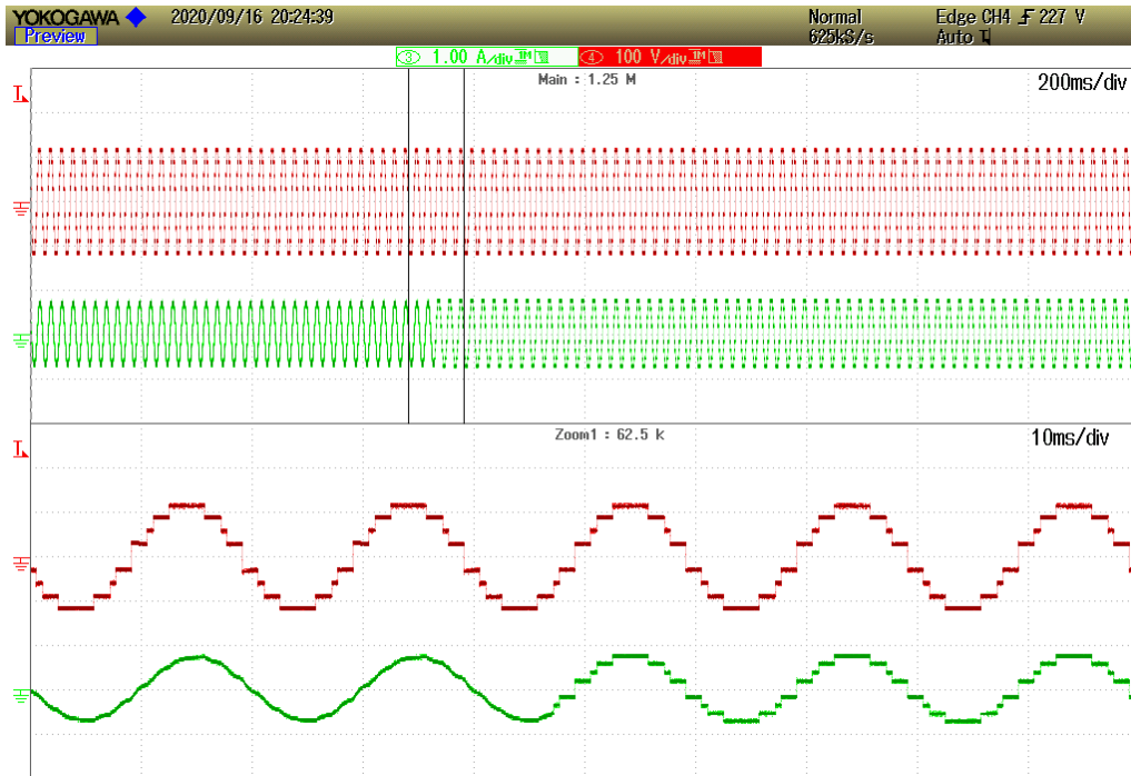
FIGURE 11. Output voltage and current waveform with change in load from RL to R load with symmetrical configuration.
