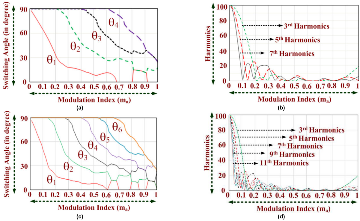
FIGURE 4. Switching angle and Harmonics (a) Optimized switching angles for 9 levels and (b) Variation of harmonics with modulation index for 9 level, (c) Optimized switching angles for 13 levels and (d) Variation of harmonics with modulation index for 13 level.
