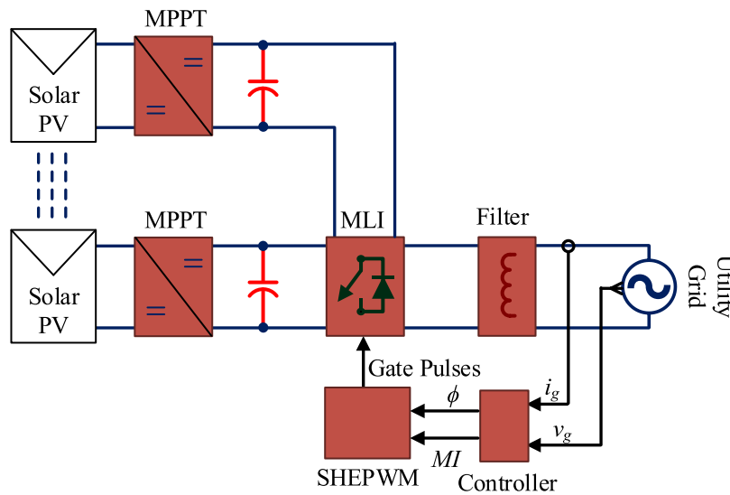
FIGURE 16. Application of the proposed topology.
