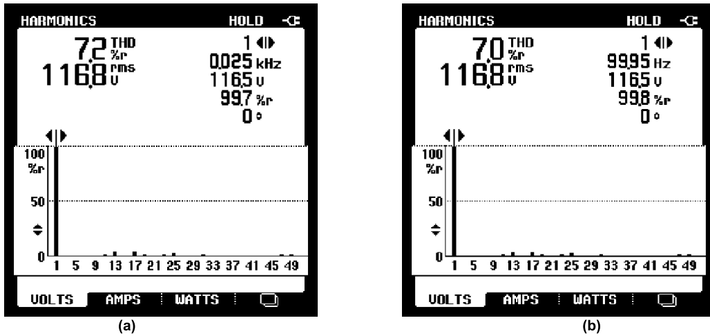
FIGURE 15. Harmonic spectrum of 13 level output voltage at modulation index of 0.69 at output frequency of (a) 25Hz and (b) 100Hz.
